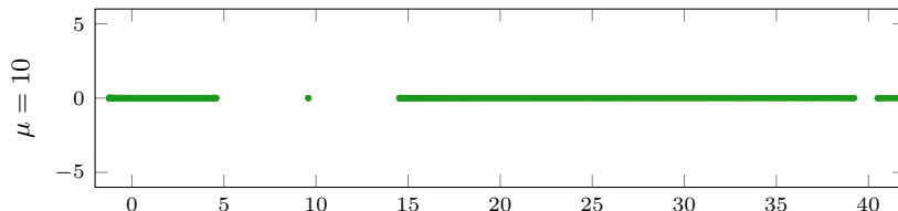
FIGURE 6. Spectral approximation from finite difference scheme on truncated domain [-100.7, 100.7] . The spurious eigenvalue in the gap for \mu = 10 can appear for arbitrarily fine discretization.
