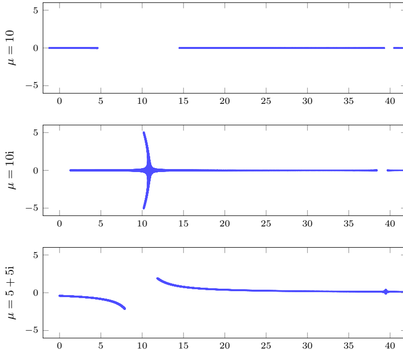
FIGURE 4. Spectral approximation in \mathbb{C} for the Mathieu operator for \mu \in \{10, 10i, 5 + 5i\} . Parameter values: N = 200 , z_0 = 45 , n = 50 , C = 2 \cdot 10^{-5} .
