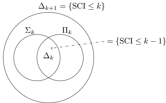
FIGURE 1. The SCI Hierarchy for k \in \{1, 2, 3\} .
