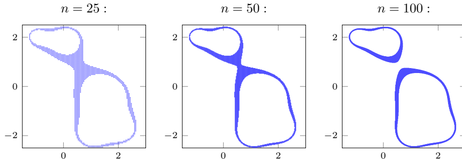
FIGURE 2. Output of \Gamma_n(A) in the complex plane for different values of n .
