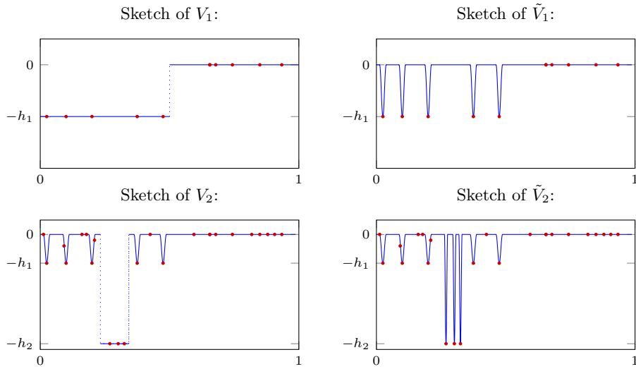
FIGURE 3. Sketch the first few iterations V_k , \tilde{V}_k . The red dots represent the points x_i , which represent the information in \Lambda_{\Gamma_n} .
