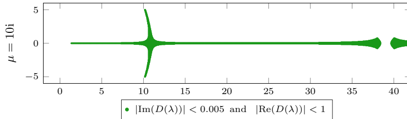
FIGURE 5. Spectral approximation with discriminant method.
