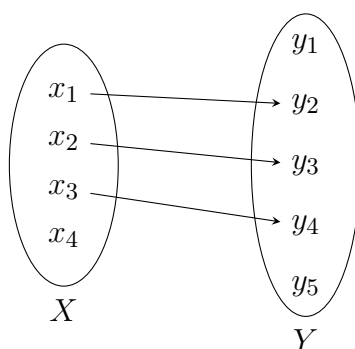
Figure 2.2: An injective ( 1-1 ) function
